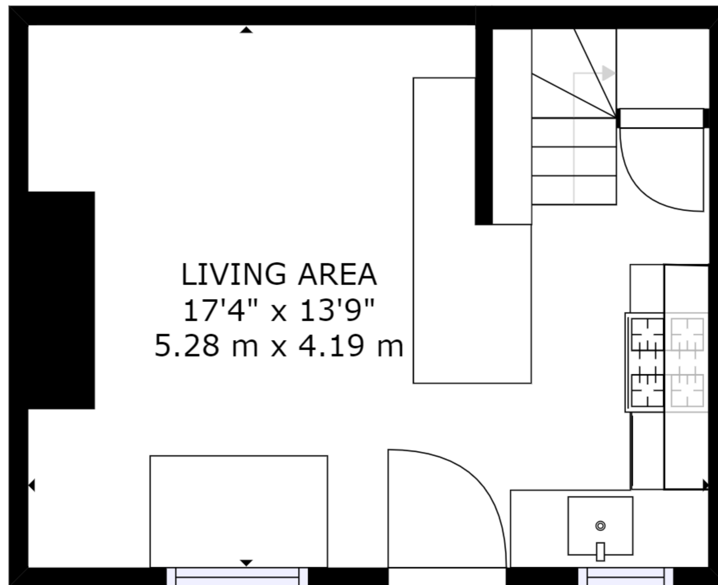
FLOOR 1
