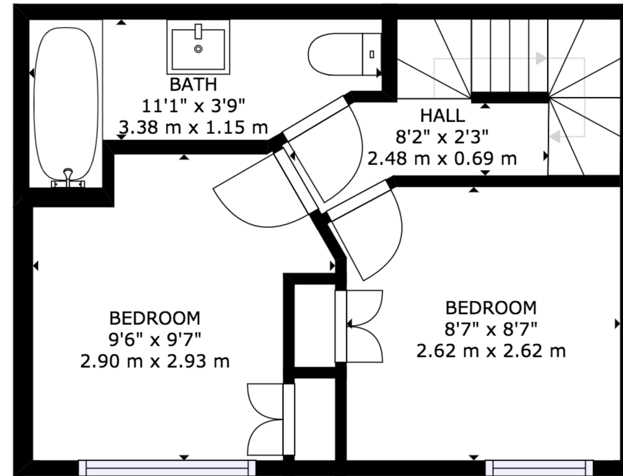
FLOOR 3
